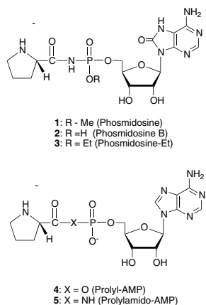
Figure 1. Various derivative of phosmidosine and prolyl-AMP.
